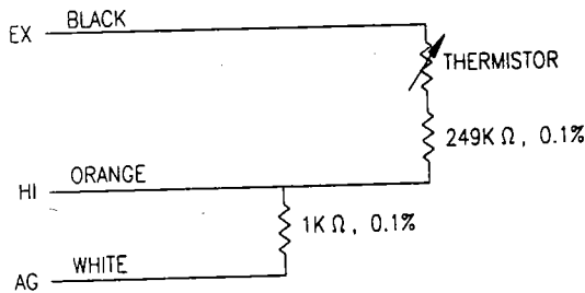
FIGURE 5. Thermistor Probe Schematic
