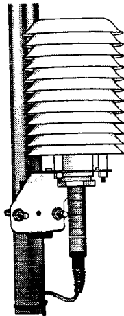
FIGURE 2. HMP35C and 41002 Radiation Shield on a CM6/CM10 Tripod Mast or UT10 Tower Leg
