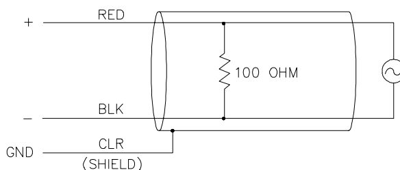
Figure 1. LI200S Schematic
