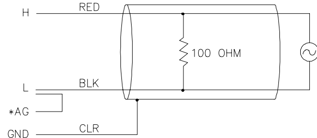
Figure 2. Differential Measurement Connection
