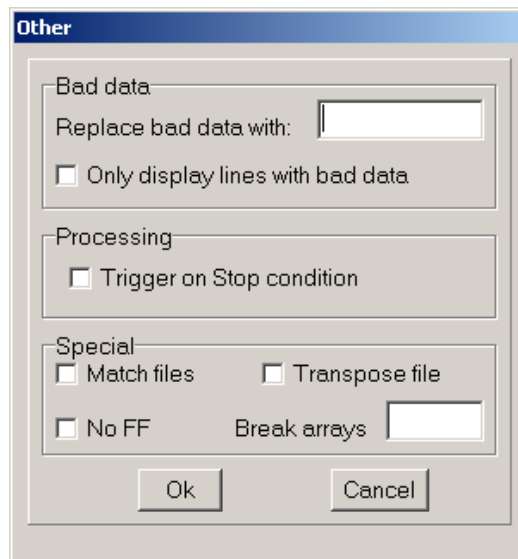
FIGURE 10.3-2. Other Output File Options
